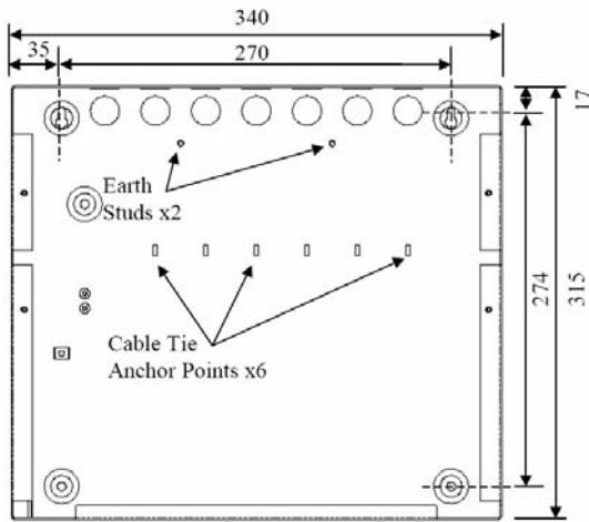
Enclosure Size and Fixing Point Dimensions
